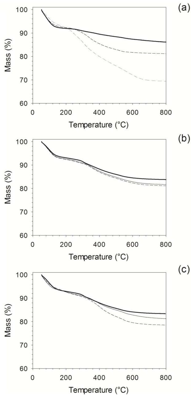
Figure 4. Thermal Gravimetric Analysis (TGA) of silica nanocarriers unfunctionalised (a), amino functionalised (b) and succinylated (c).
